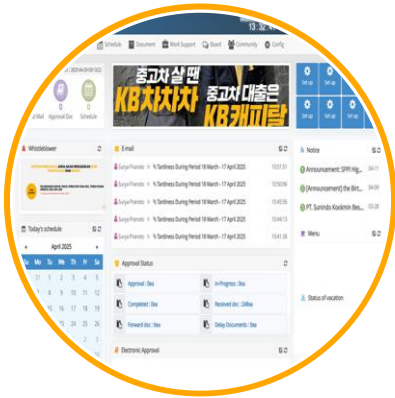
Groupware
